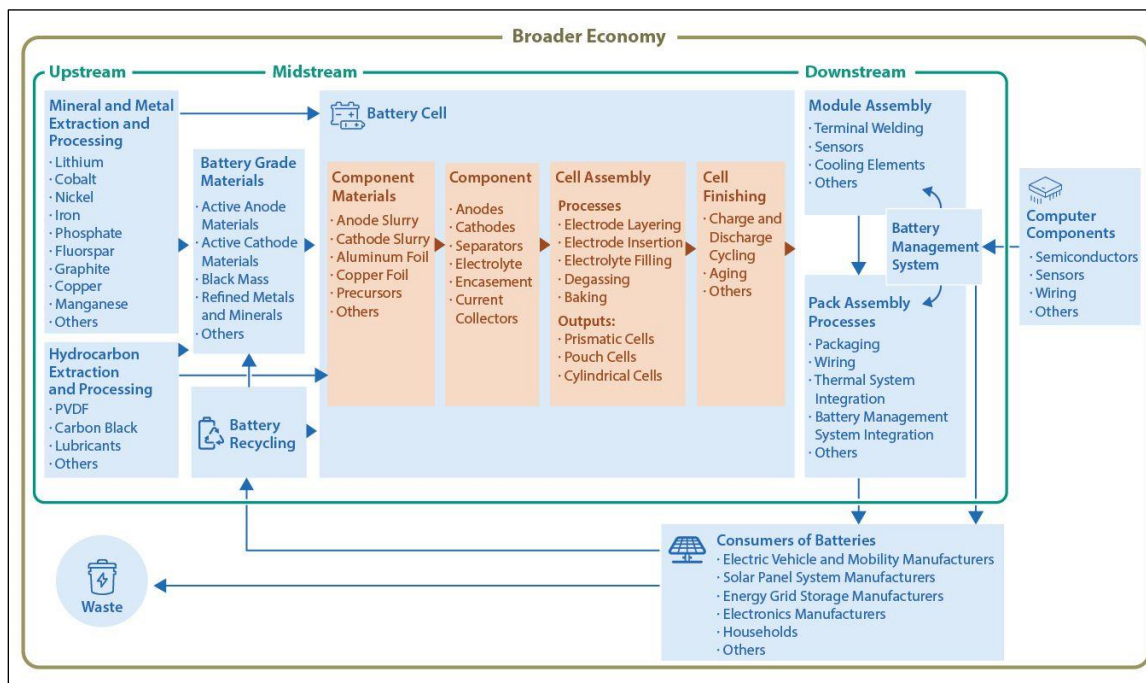
Figure 9. Lithium-Ion Battery Supply Chain
