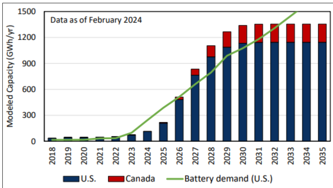
Figure 11. Projected Lithium-Ion Cell Production Capacity
