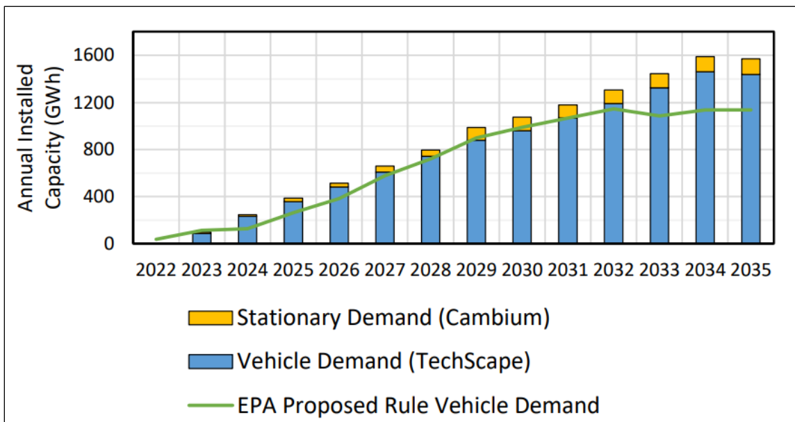
Figure 10. U.S. Lithium-Ion Projected Battery Demand
