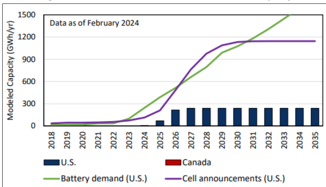
Figure 12. Aluminum Current Collector Foil Planned Capacity
