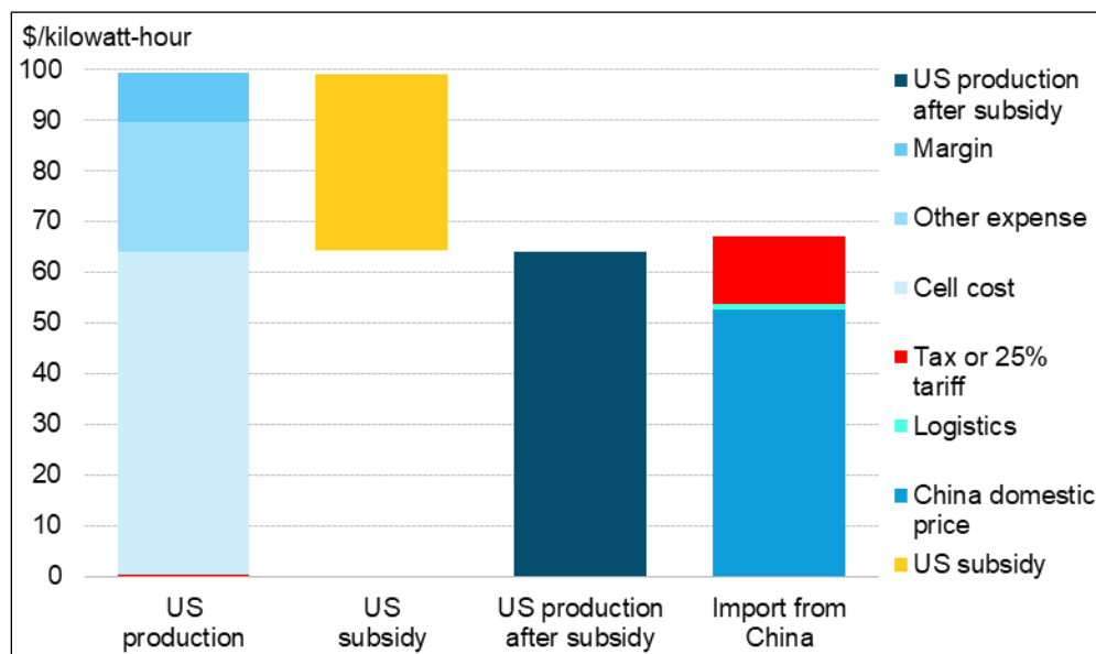
Figure 5. Lithium-Iron-Phosphate Battery Price Comparison
