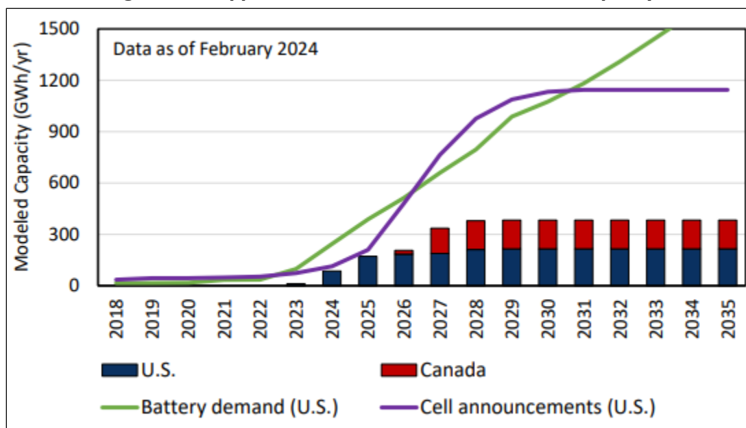
Figure 13. Copper Current Collector Foil Planned Capacity
